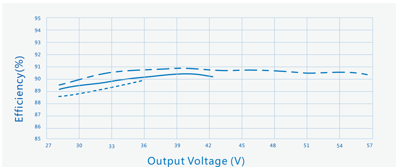
Efficiency Vs. Output Voltage (Vin=120Vac)
